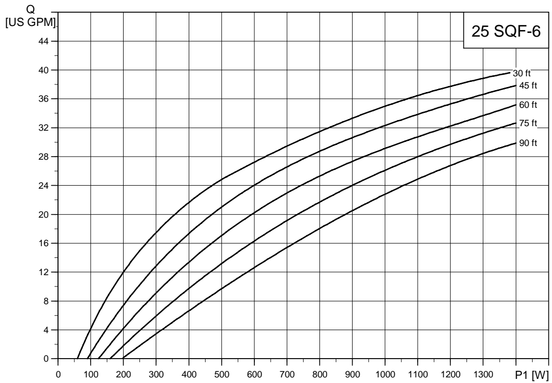
Fig. 33 Curve chart, 25 SQF-6
