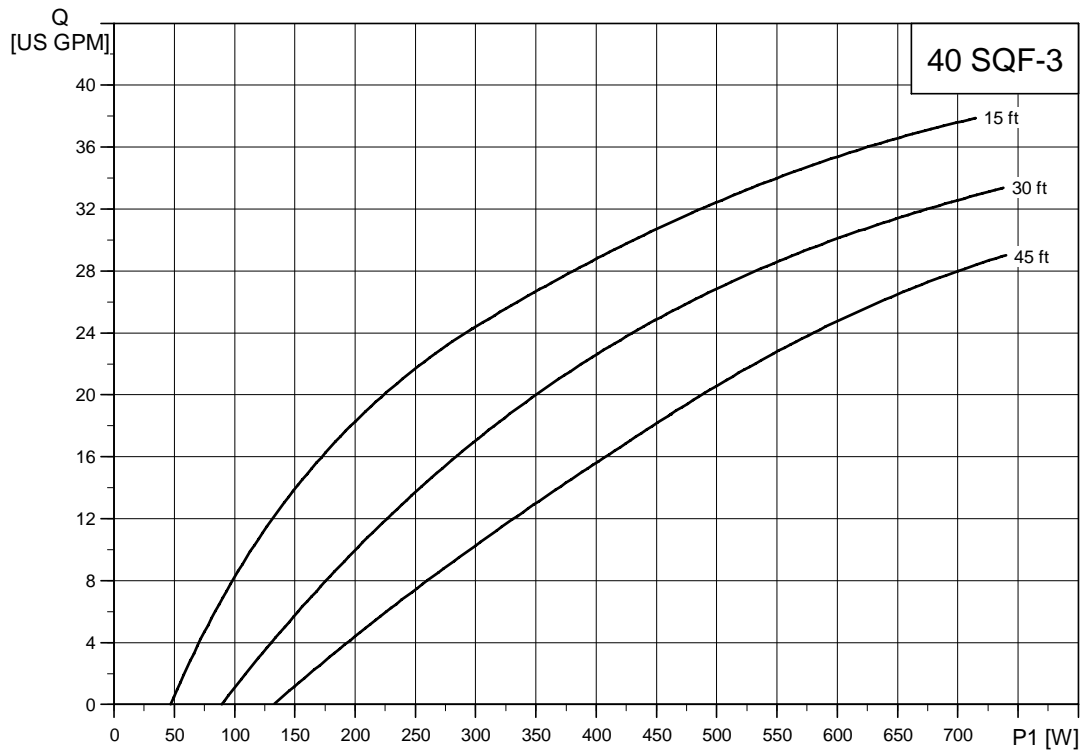
Fig. 34 Curve chart, 40 SQF-3
