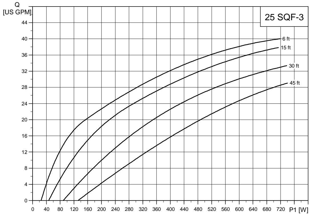
Fig. 32 Curve chart, 25 SQF-3
