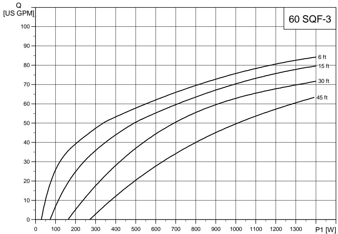
Fig. 36 Curve chart, 60 SQF-3
