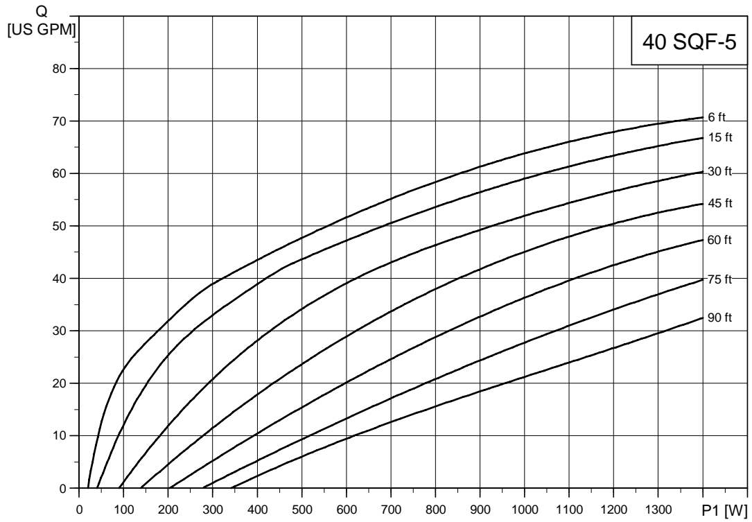
Fig. 35 Curve chart, 40 SQF-5
