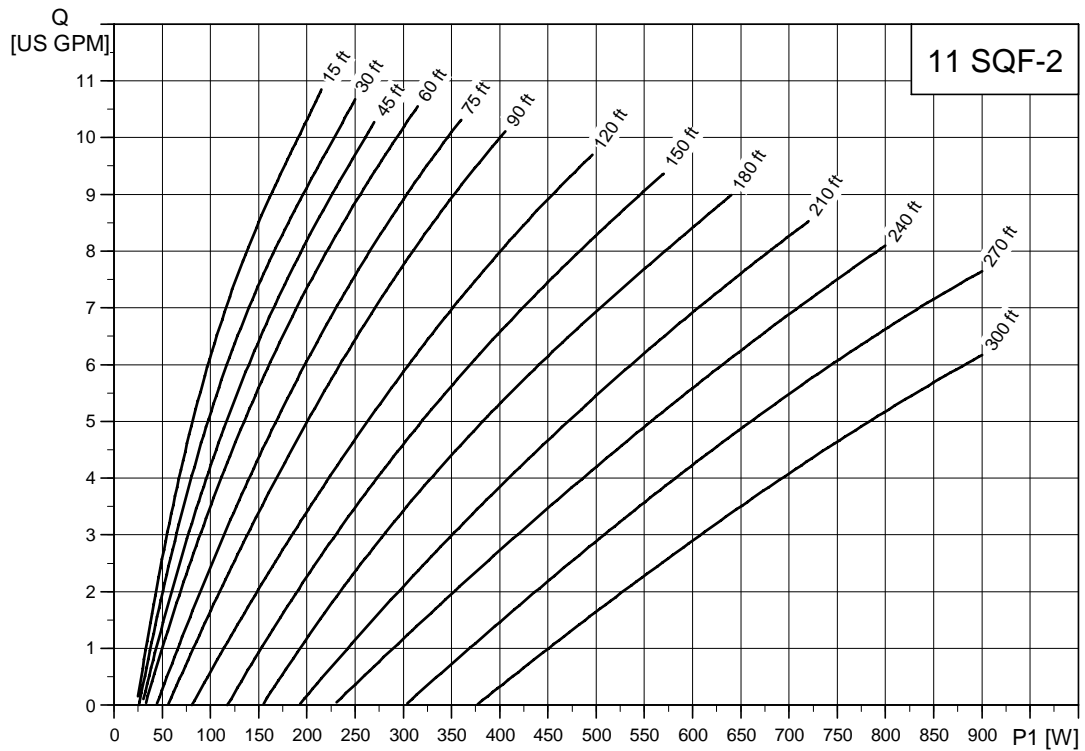
Fig. 30 Curve chart, 11 SQF-2
