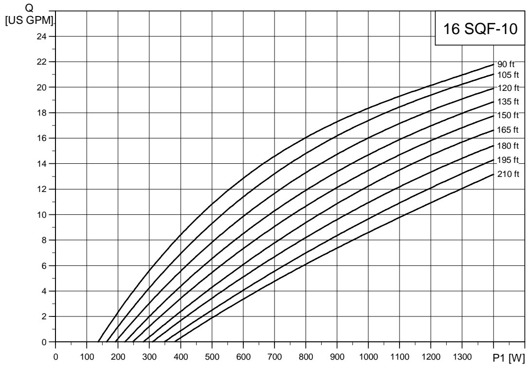
Fig. 31 Curve chart, 16 SQF-10
