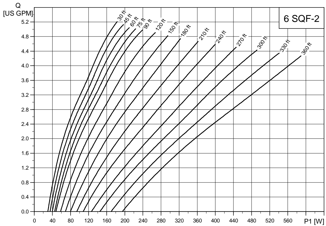
Fig. 29 Curve chart, 6 SQF-2
